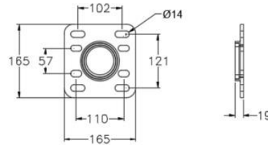
OFF-SIDE MOUNTING BRACKET W/ BUSHING
